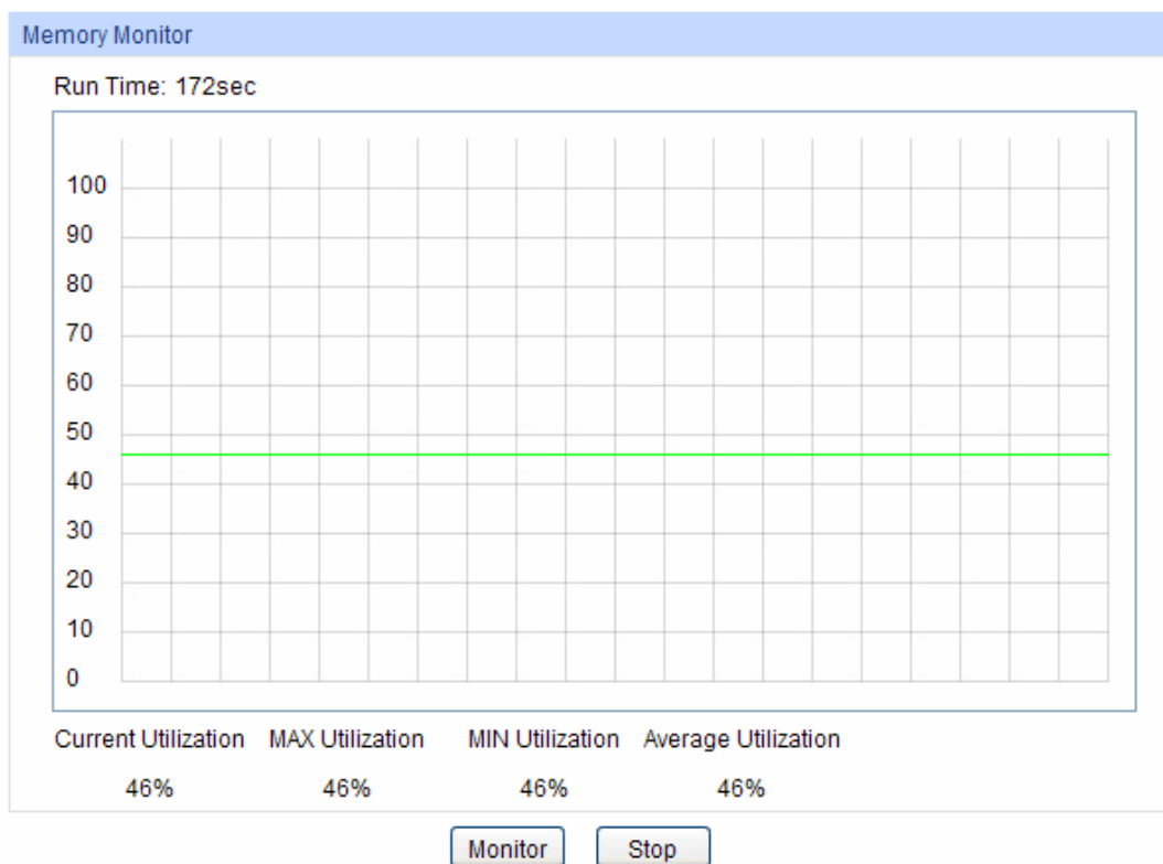
Figure 12-2 Memory Monitor
